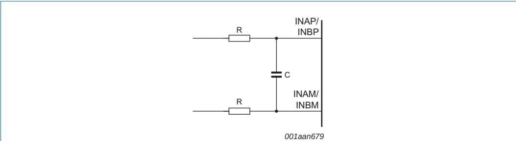
Fig 17. Anti-kickback circuit
